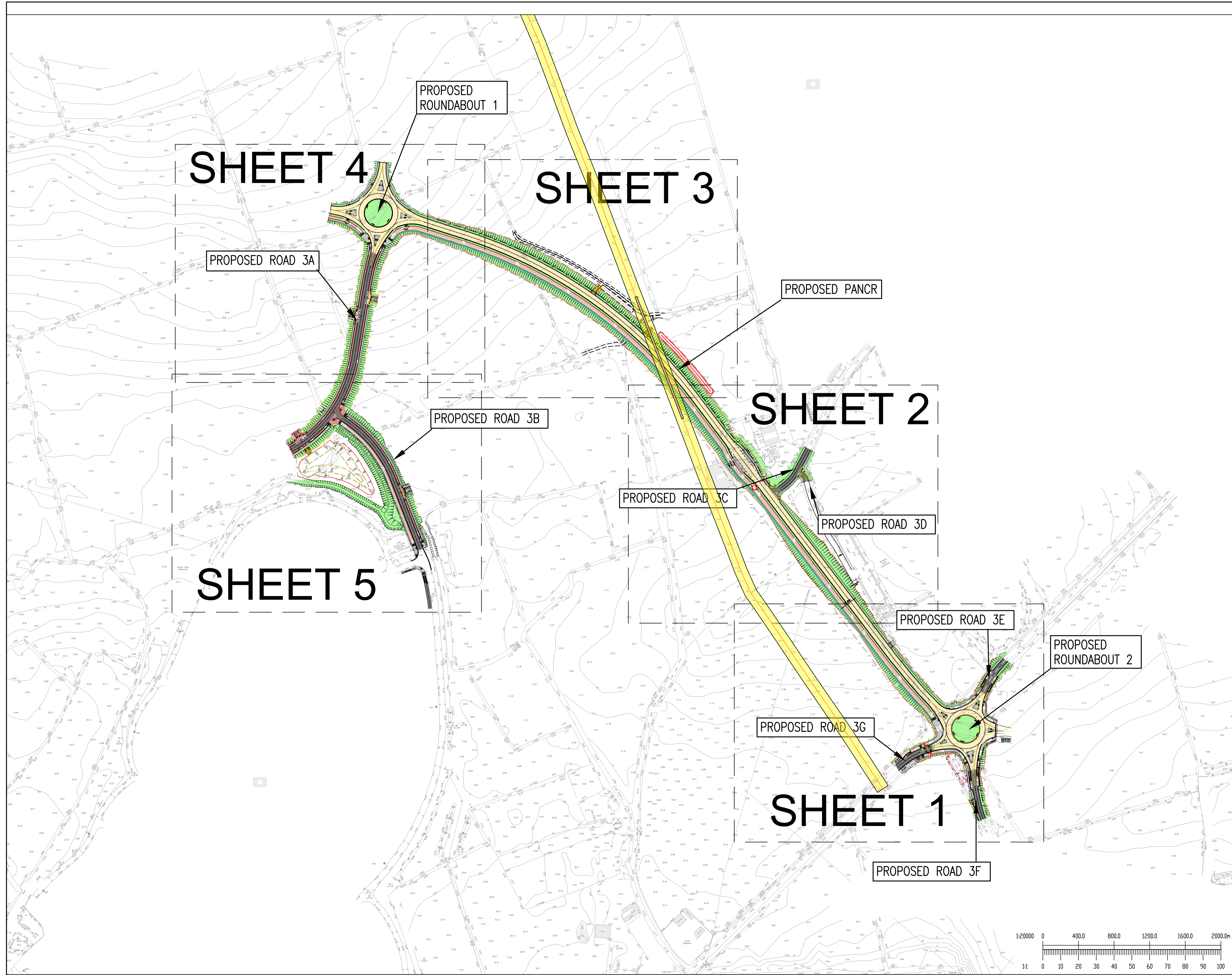
PLAN VIEW - PROPOSED ROADS LAYOUT AND LEVELS - GENERAL ARRANGEMENT PLAN SCALE 1:2000 ©A1
